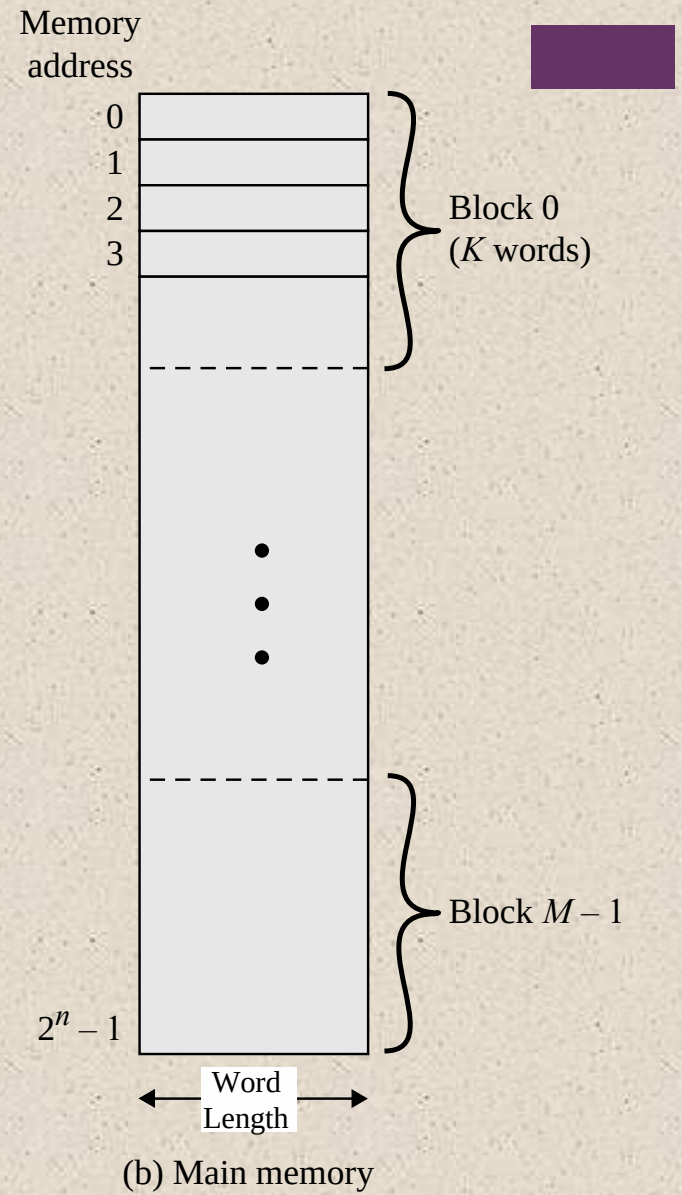
Figure 4.4 Cache/Main-Memory Structure
